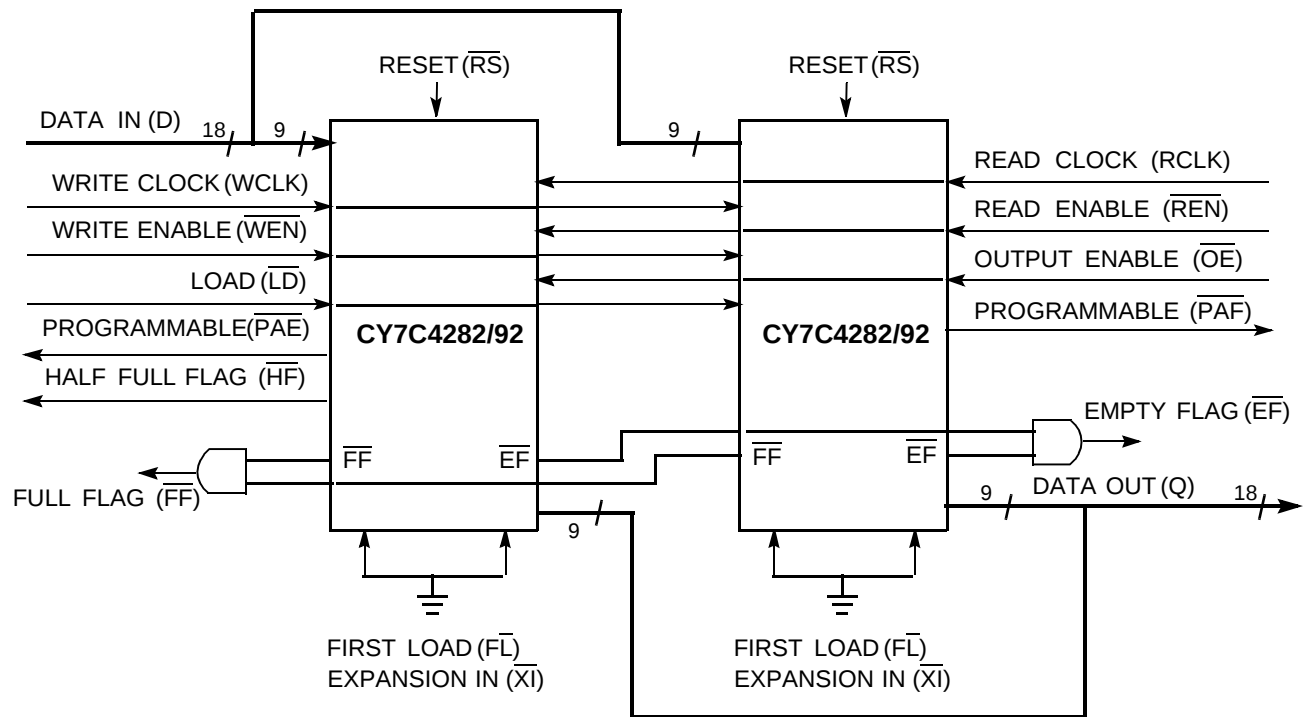
Figure 2. Block Diagram of 64K × 9/128K × 9 1M Deep Sync FIFO Memory Used in a Width Expansion Configuration
