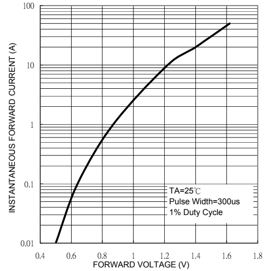
FIG. 3 TYPICAL FORWARD CHARACTERISRICS
