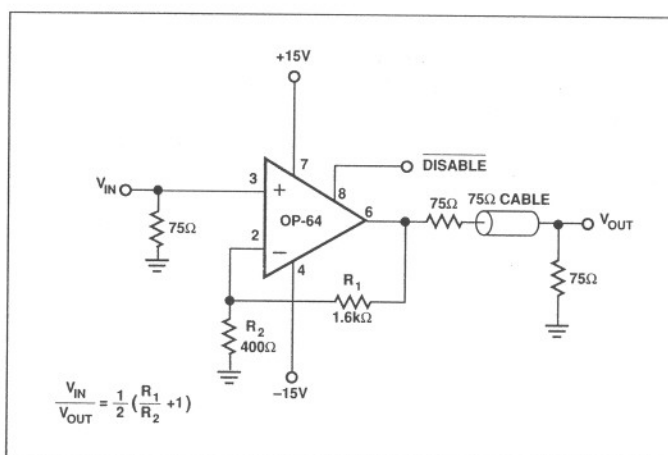
FIGURE 8: Video Amplifier/Terminated Line Driver
