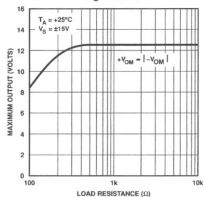
MAXIMUM OUTPUT VOLTAGE vs LOAD RESISTANCE V_S = \pm 15\text{V}
