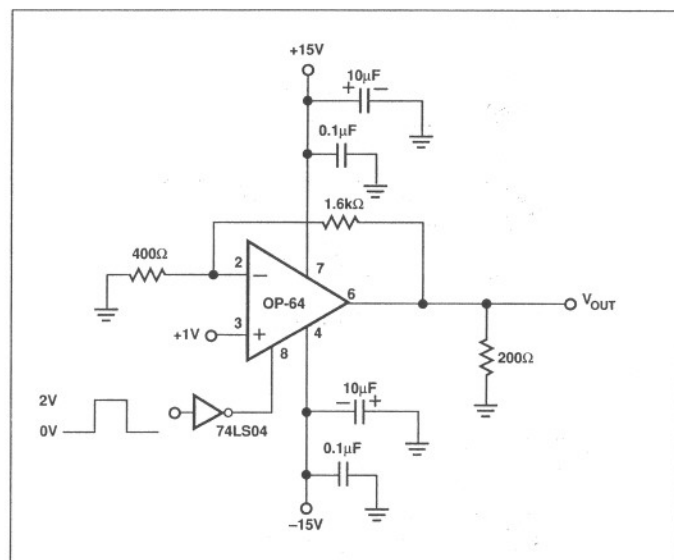
FIGURE 4: DISABLE Turn-On/Turn-Off Test Circuit
