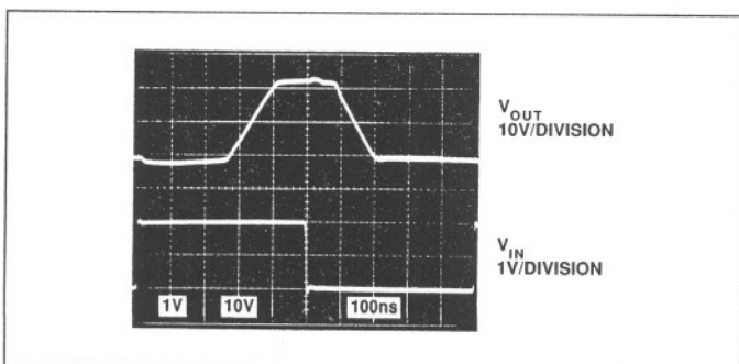
FIGURE 6: OP-64 Overdrive Recovery
