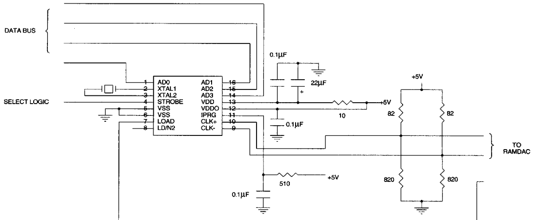
ICS1562A-001 Typical Interface
