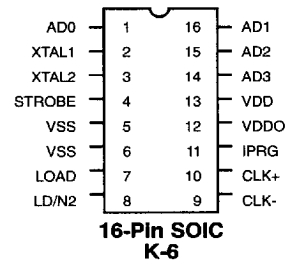
ICS1562A - 001 Pinout
