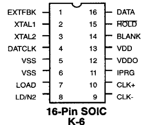
ICS1562A - 201 Pinout
