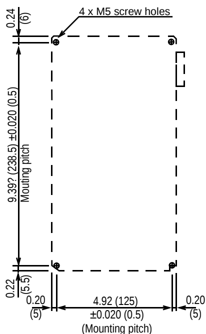
Mounting Hole Diagram
