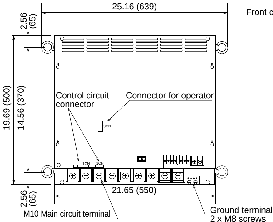
Mounting Hole Diagram
