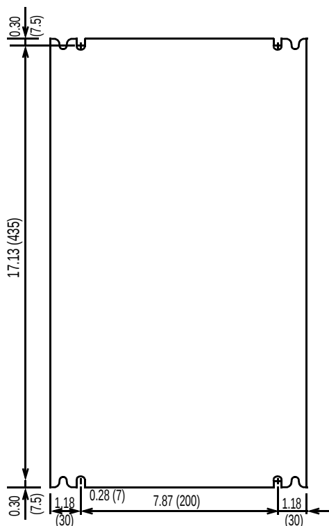
Mounting Hole Diagram
