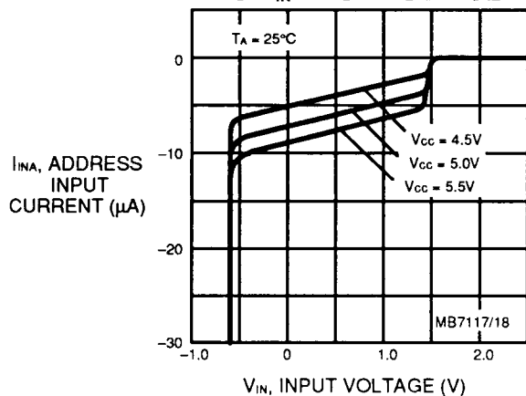
Fig. 6 – I_{INA} INPUT CURRENT vs. V_{IN} INPUT VOLTAGE
