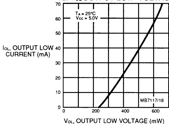
Fig. 8 – I_{OL} OUTPUT LOW CURRENT vs. V_{OL} OUTPUT LOW VOLTAGE
