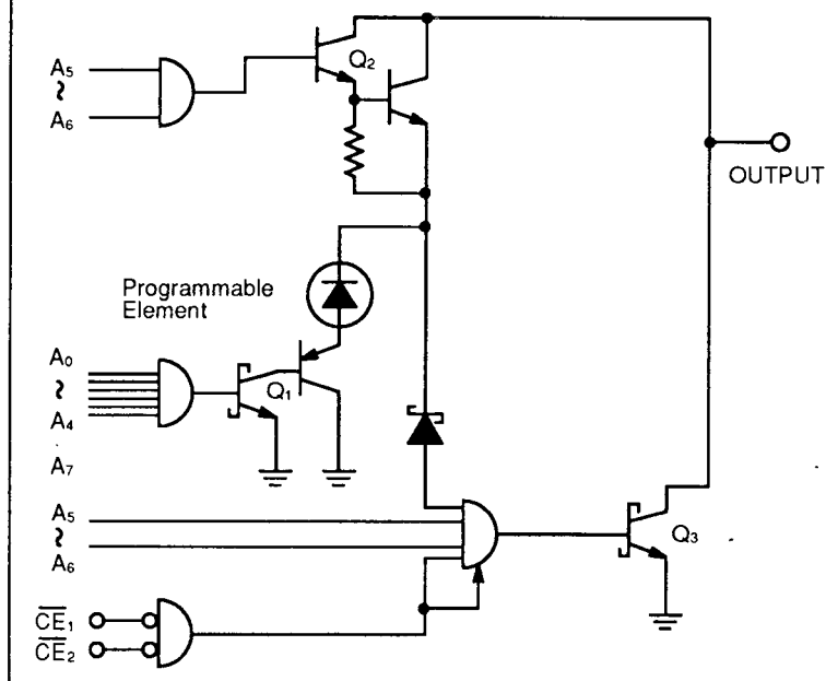
Fig. 25 – INTERNAL PROGRAMMING CIRCUIT
