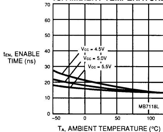
Fig. 21 – t_{EN} ENABLE TIME vs. AMBIENT TEMPERATURE
