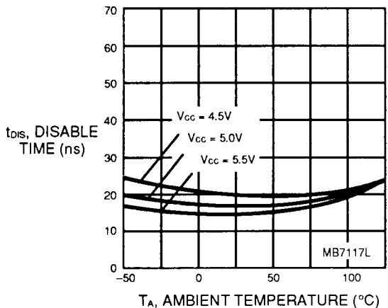
Fig. 16 – t_{DIS} DISABLE TIME vs. AMBIENT TEMPERATURE
