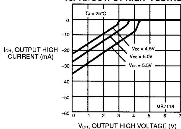
Fig. 9 – I_{OH} OUTPUT HIGH CURRENT vs. V_{OH} OUTPUT HIGH VOLTAGE
