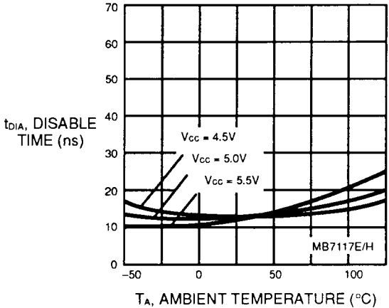
Fig. 14 – t_{DIS} DISABLE TIME vs. AMBIENT TEMPERATURE
