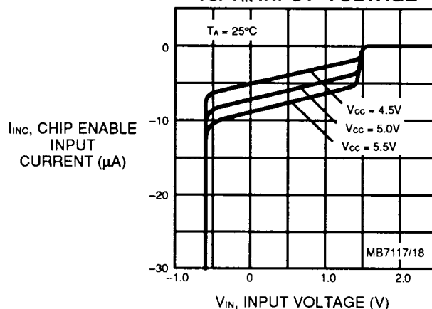
Fig. 7 – I_{INC} INPUT CURRENT vs. V_{IN} INPUT VOLTAGE
