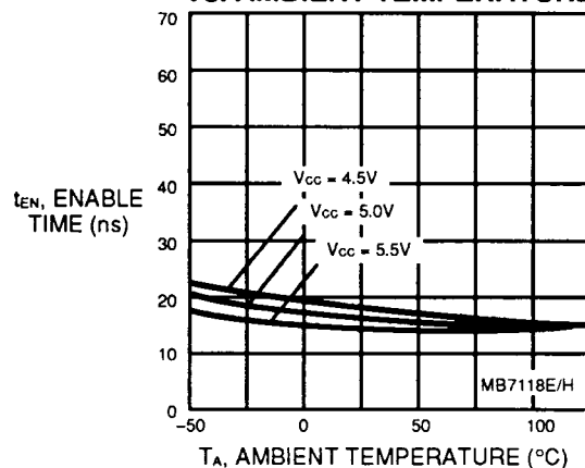
Fig. 19 – t_{EN} ENABLE TIME vs. AMBIENT TEMPERATURE
