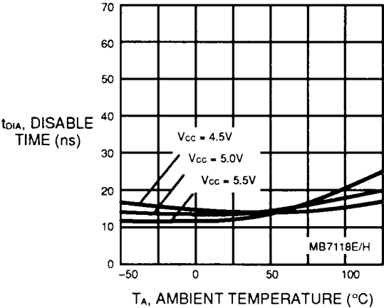
Fig. 15 – t_{DIS} DISABLE TIME vs. AMBIENT TEMPERATURE
