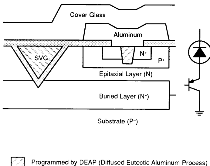
Fig. 24 – PROGRAMMED CELL (CROSS SECTION)
