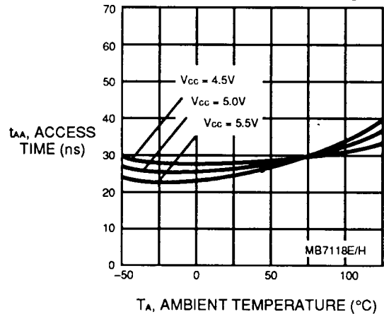
Fig. 11 – t_{AA} ACCESS TIME vs. AMBIENT TEMPERATURE
