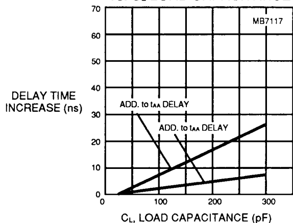
Fig. 22 – DELAY TIME INCREASE vs. C_L LOAD CAPACITANCE
