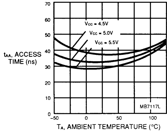
Fig. 12 – t_{AA} ACCESS TIME vs. AMBIENT TEMPERATURE
