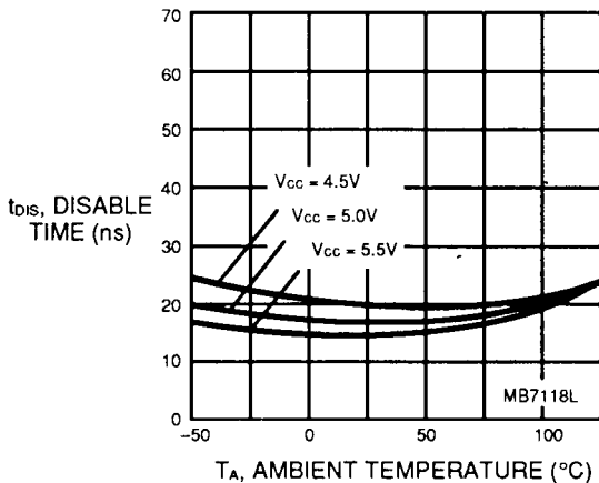
Fig. 17 – t_{DIS} DISABLE TIME vs. AMBIENT TEMPERATURE
