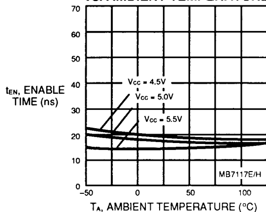
Fig. 18 – t_{EN} ENABLE TIME vs. AMBIENT TEMPERATURE
