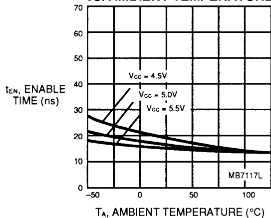
Fig. 20 – t_{EN} ENABLE TIME vs. AMBIENT TEMPERATURE
