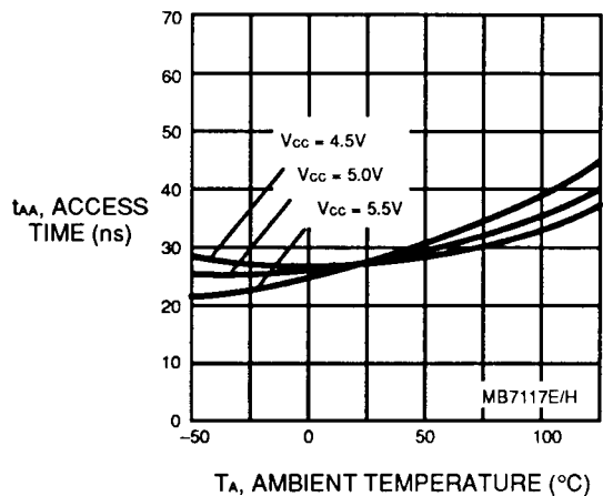
Fig. 10 – t_{AA} ACCESS TIME vs. AMBIENT TEMPERATURE
