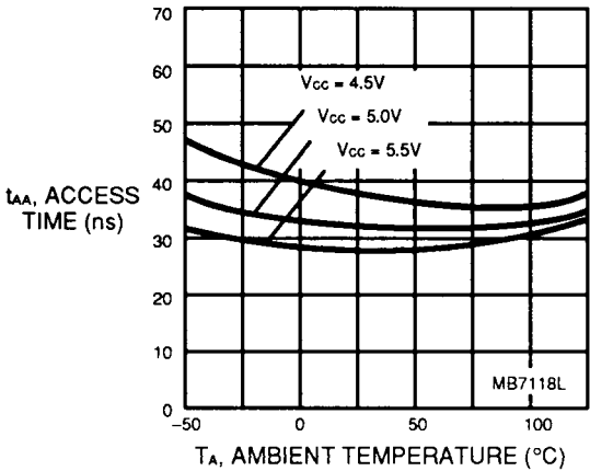
Fig. 13 – t_{AA} ACCESS TIME vs. AMBIENT TEMPERATURE
