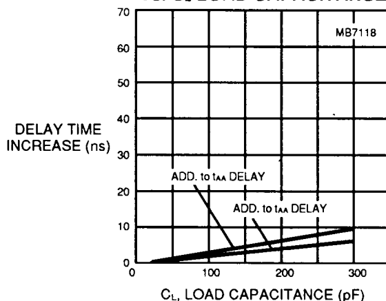
Fig. 23 – DELAY TIME INCREASE vs. C_L LOAD CAPACITANCE
