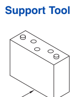
2X 1/4-20 UNC-2B MOUNTING HOLES
