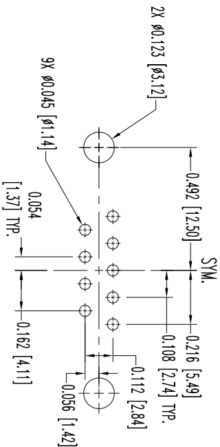
CONTACT HOLE PATTERN
