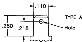
Mating .110 series tab Dimensions type A
