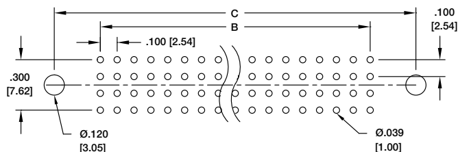
Recommended PCB Layout - Female
