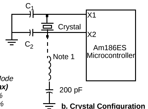
Figure 8. Am186ES and Am188ES Microcontrollers Oscillator Configurations
