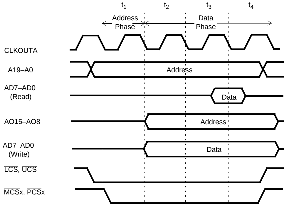
Figure 7. Am188ES Microcontroller—Read and Write with Address Bus Disable In Effect
