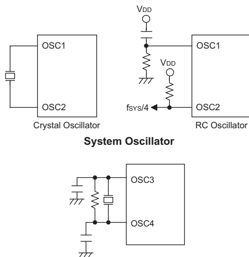
32768Hz Crystal/RTC Oscillator
