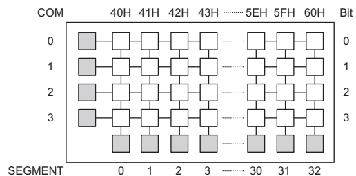
Display Memory
