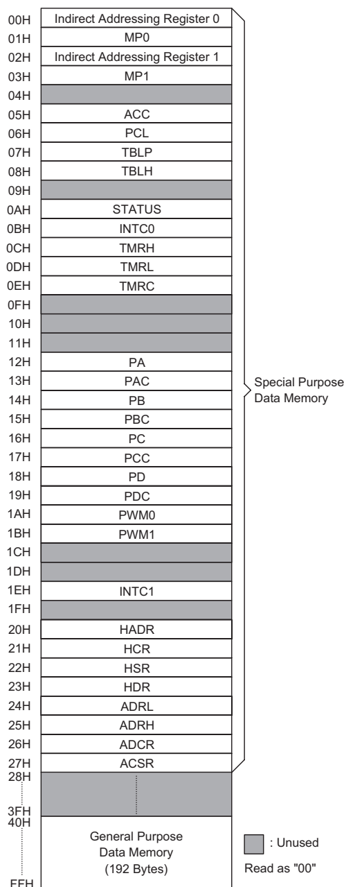
RAM Mapping
