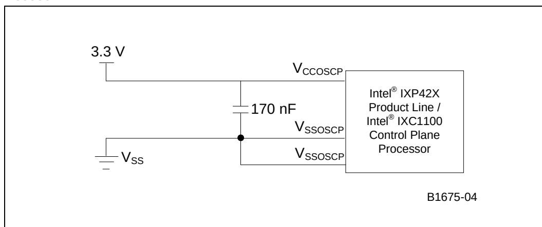
Figure 11. V_{CCSCP} Power Filtering Diagram
