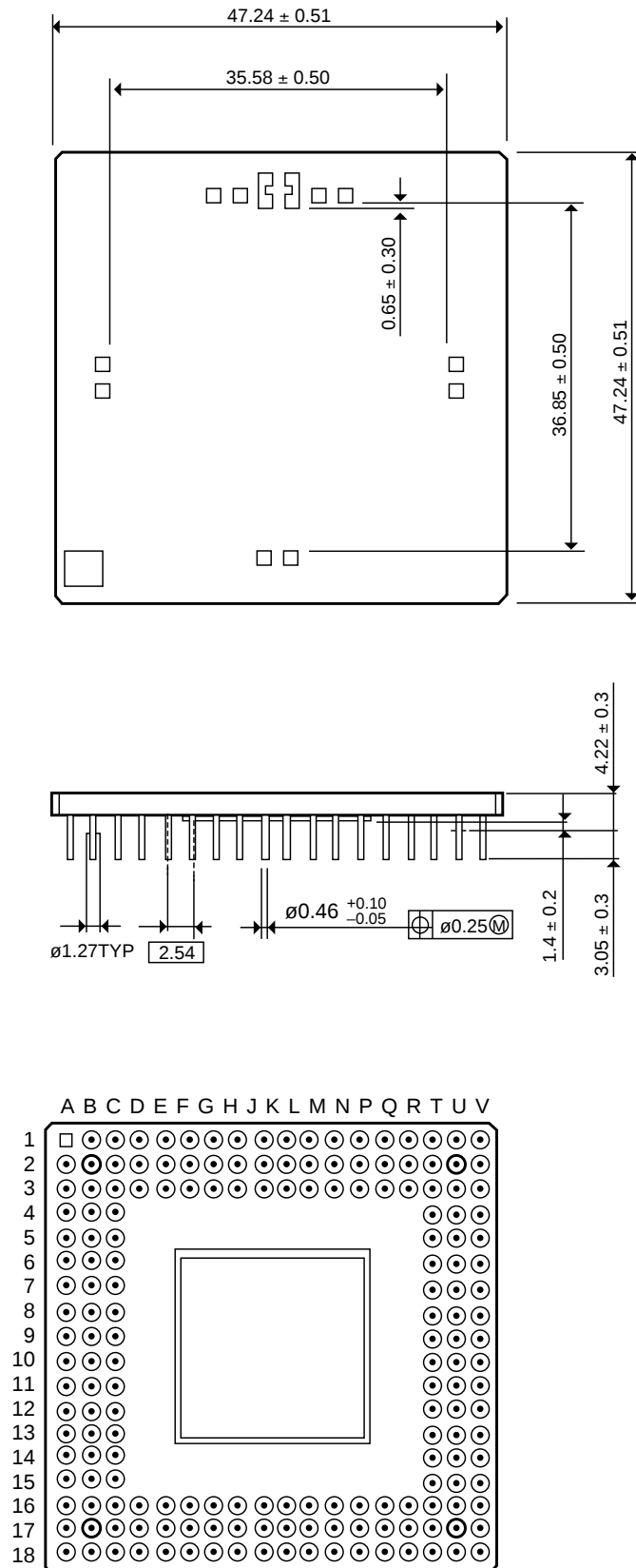
Figure 20. PGA179-C-S18D
