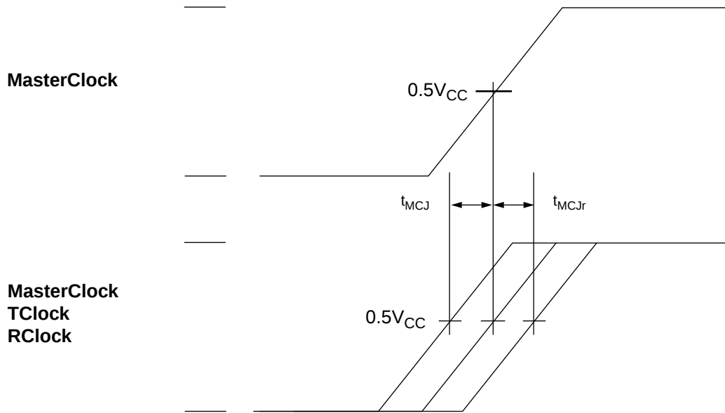
Figure 14. Clock Jitter
