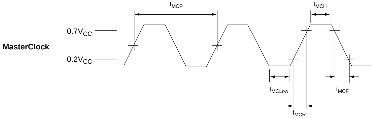
Figure 13. Clock Timing
