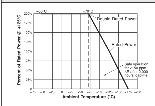
FIGURE 2 - POWER DERATING CURVE "S" SERIES
