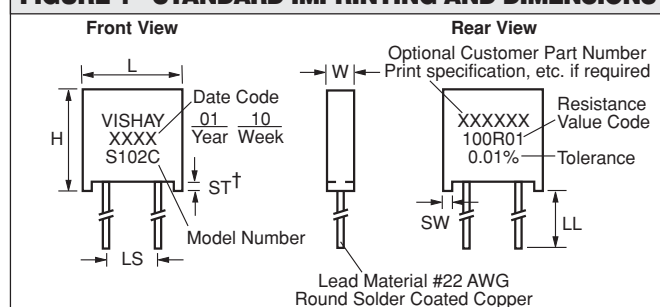
FIGURE 1 - STANDARD IMPRINTING AND DIMENSIONS
