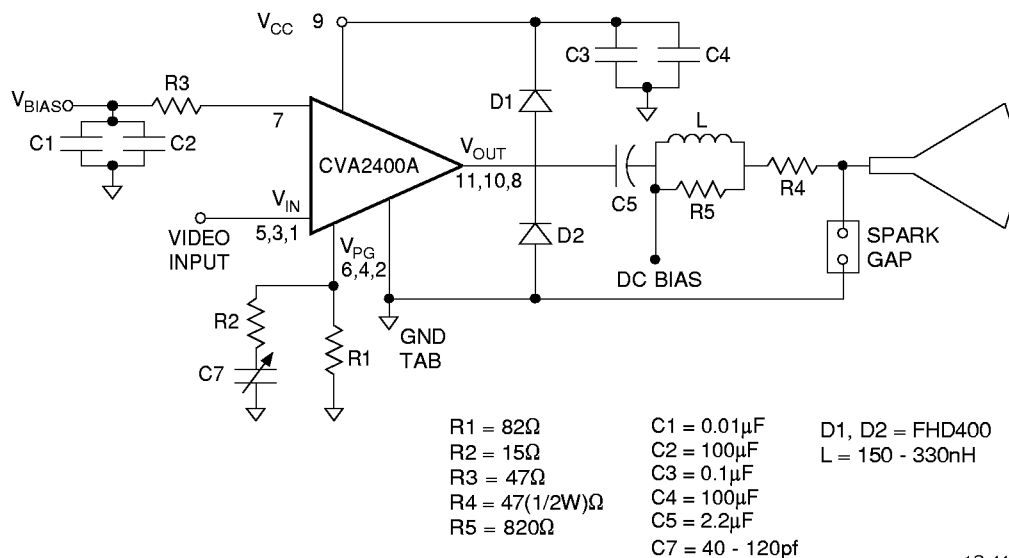
FIGURE 2. APPLICATION CIRCUIT
