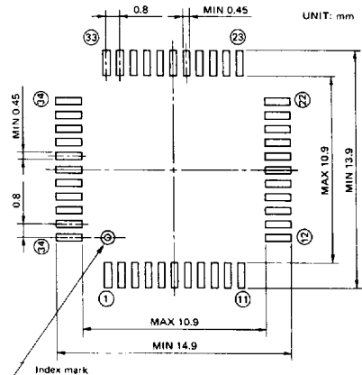
RECOMMENDED FOOTPRINT FOR QPD PACKAGE
