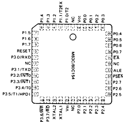
MSM83C154-XXJS/MSM80C154JS *1 (Top-View) 44 Lead Plastic Leaded Chip Carrier
