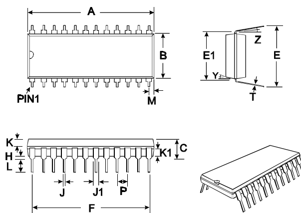
Figure 17: 24-pin SOIC Mechanical Outline: Order as part no. CMX589AD2
