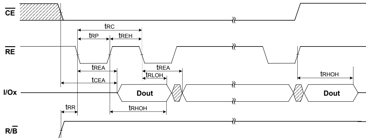
Figure 19. Serial Access Cycle after Read(EDO Type, CLE=L , \overline{WE}=H , ALE=L )
