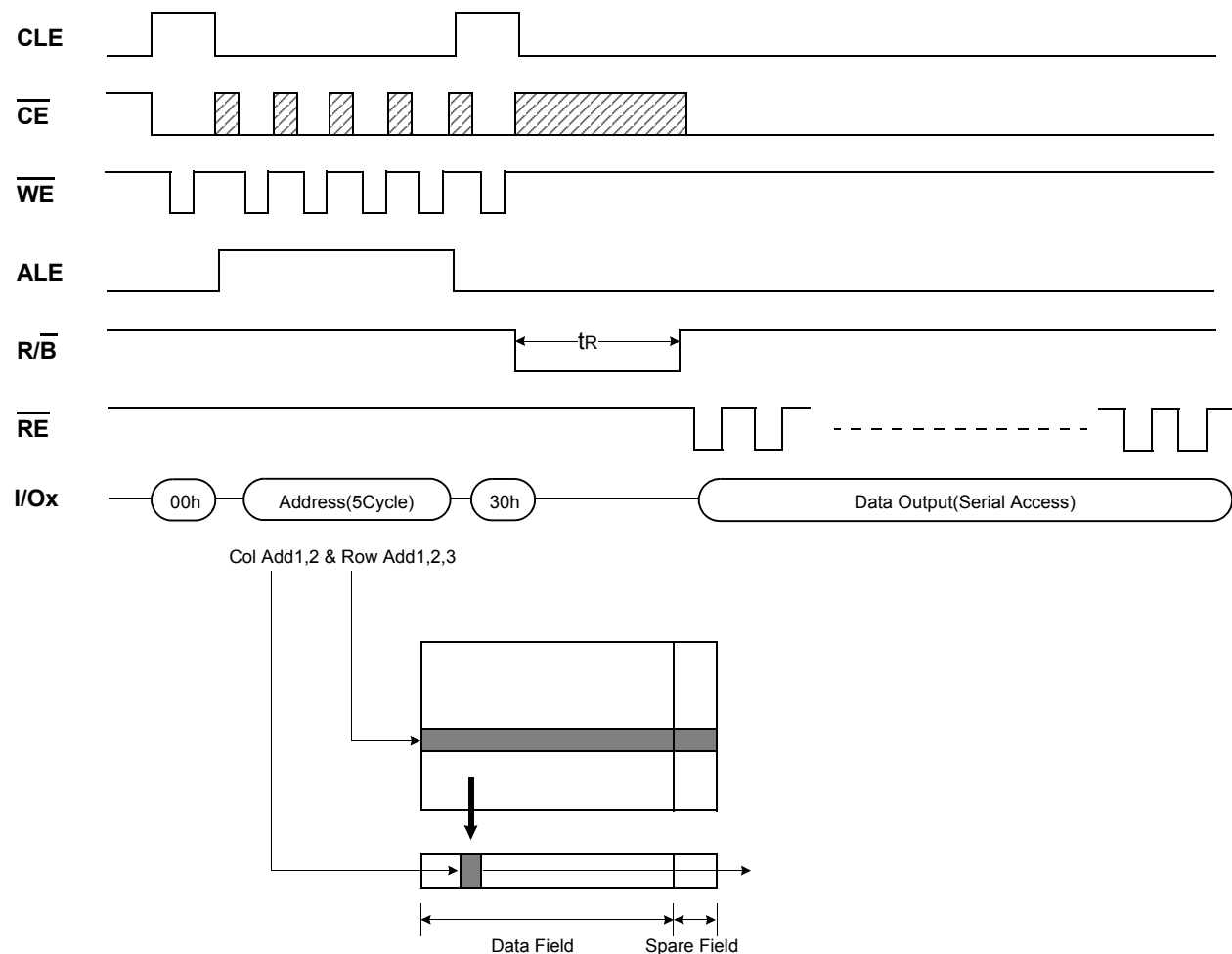
Figure 6. Read Operation
