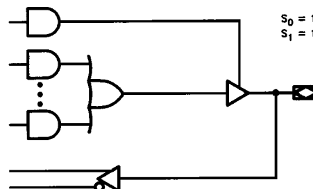
FIGURE 3-4. Combinatorial/Active High
