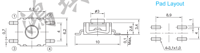
Pad Layout
