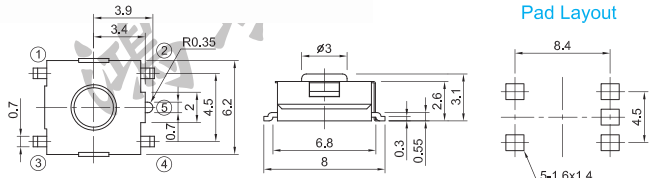
Pad Layout
