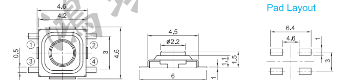
Pad Layout
