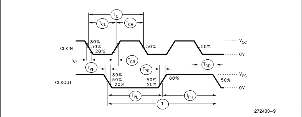
Figure 8. Input and Output Clock Waveform
