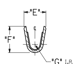
SECT. "H-H"
