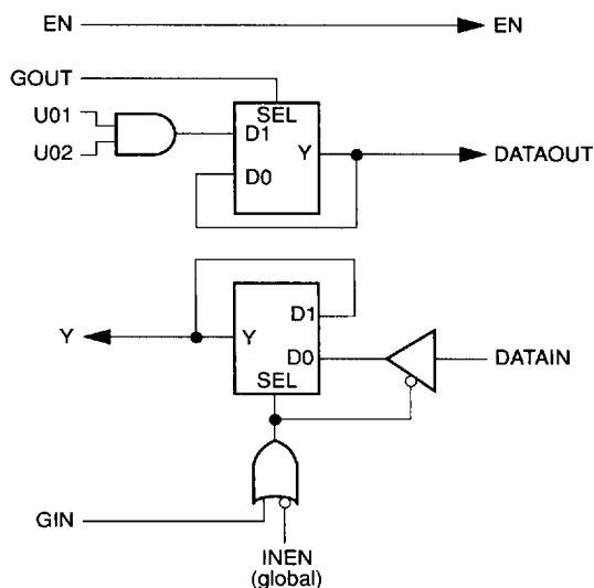
Figure 5. I/O Module
