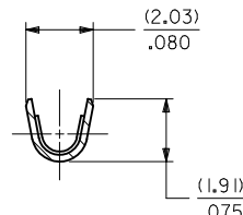
SECT. "C-C"
