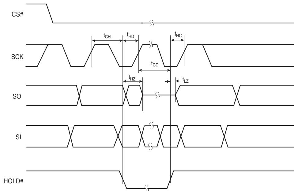
Figure 16.3 HOLD# Timing
