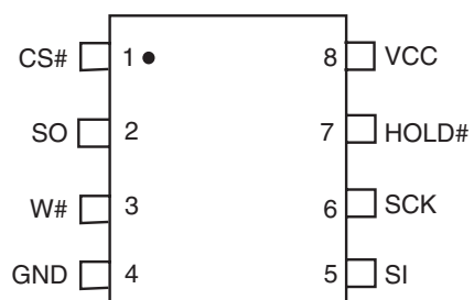
Figure 2.2 8-pin Plastic Small Outline Package (SO)
