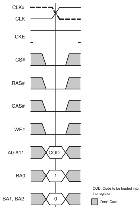
FIGURE 6 Extended Mode Register Set Command
