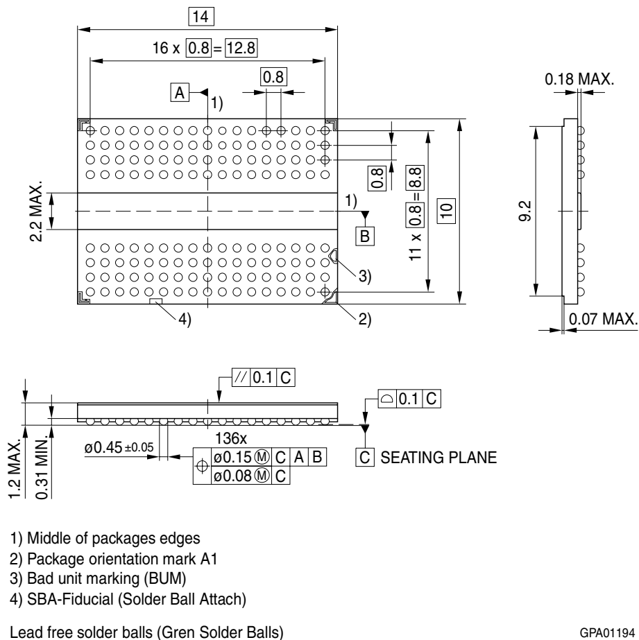
FIGURE 18 Package Outline PG-TFBGA-136-054
