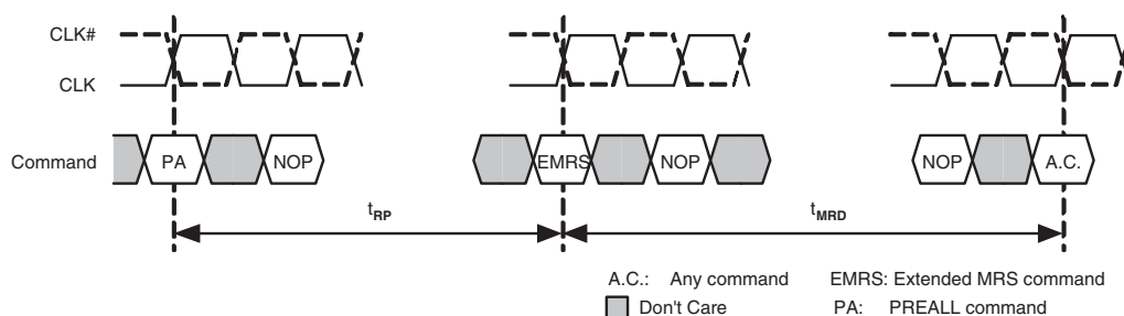
FIGURE 9 Extended Mode Register Set Timing
