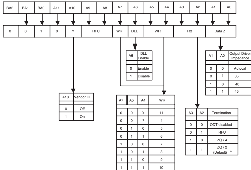
FIGURE 7 Extended Mode Register Bitmap for Mid-Range-Speed Application
