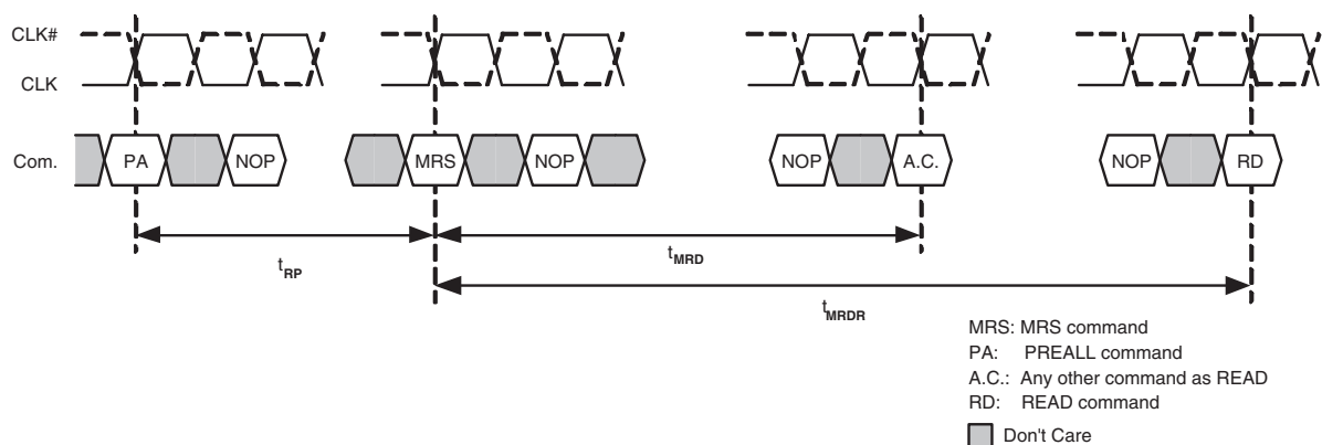
FIGURE 5 Mode Register Set Timing
