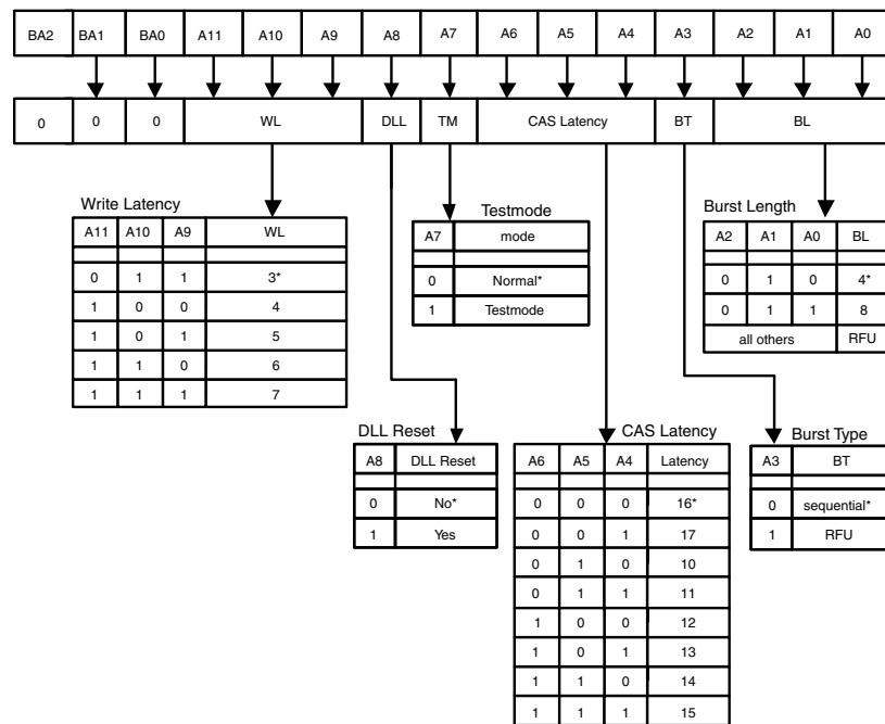
FIGURE 4 Mode Register Bitmap for High-Speed Application
