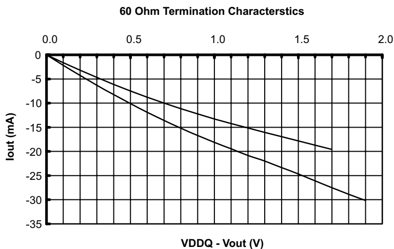
FIGURE 15 60 Ohm Active Termination Characteristic
