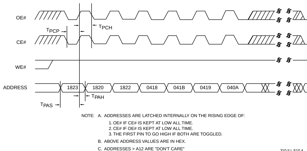
FIGURE 11: SOFTWARE DATA PROTECT DISABLE TIMING DIAGRAM
