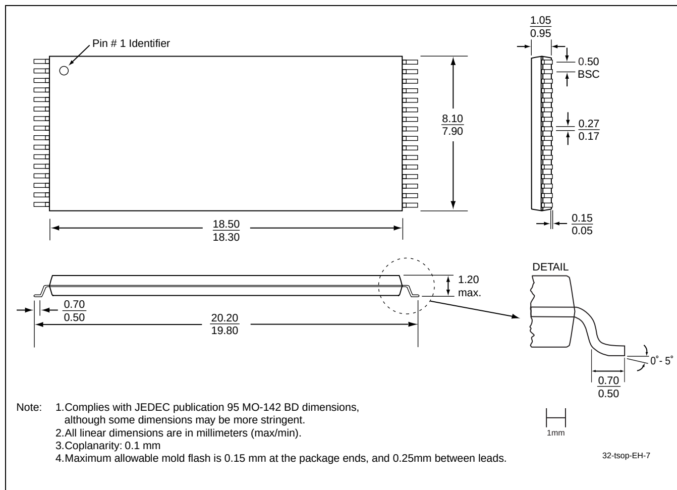
32-LEAD THIN SMALL OUTLINE PACKAGE (TSOP) 8MM X 20MM GREENLIANT PACKAGE CODE: EH
