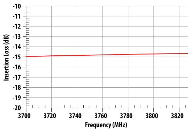
Figure 5. Rejection at Tx Second Harmonic
