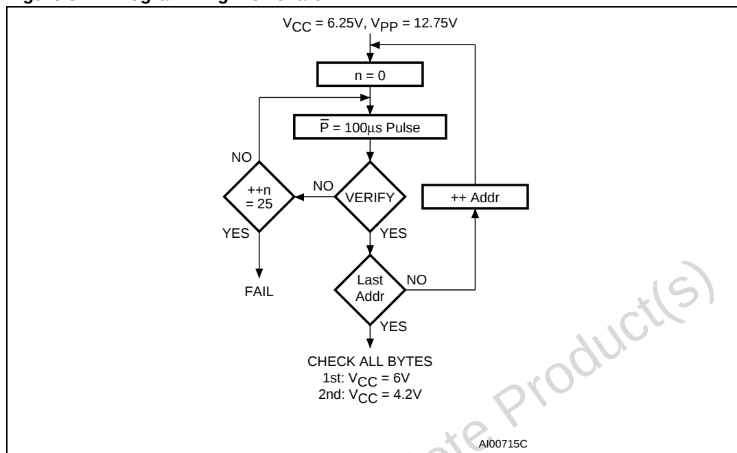
Figure 5. Programming Flowchart
