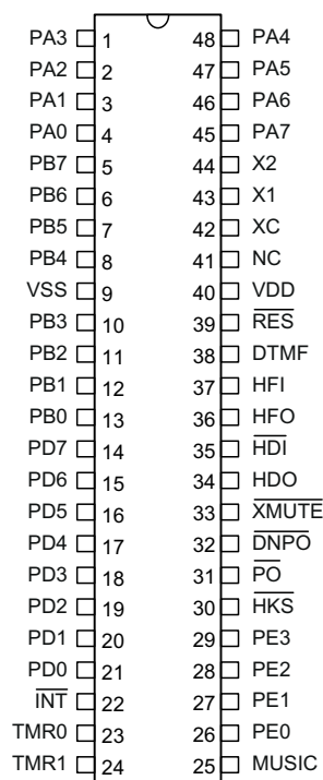
HT95A200/20P/300/30P – 48 SSOP-A
