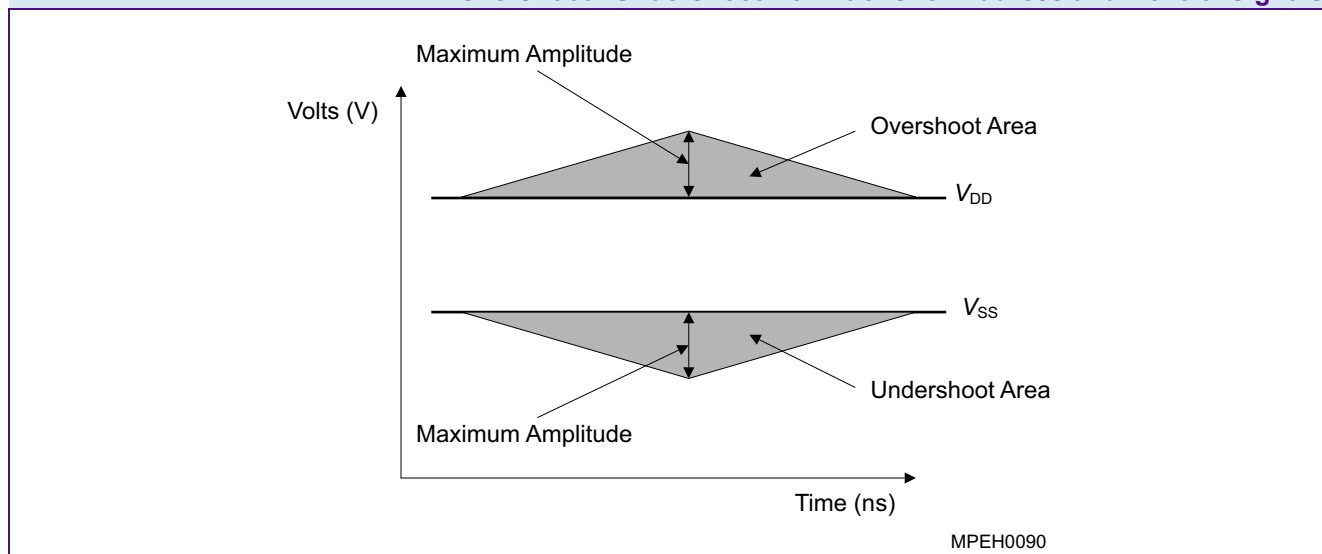
AC Overshoot / Undershoot Definitions for Address and Control Signals
