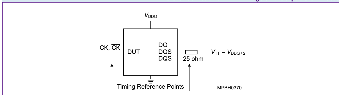
FIGURE 4 Reference Load for AC Timings and Output Slew Rates
