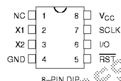
8-PIN DIP
