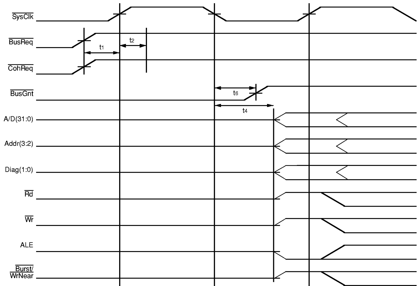
Figure 26. End of Coherent DMA Request
