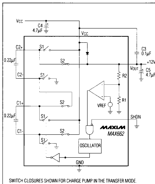
Figure 1. Block Diagram
