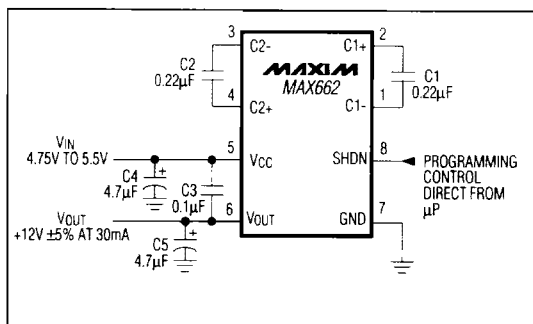
Figure 3. Flash EEPROM programming power supply
