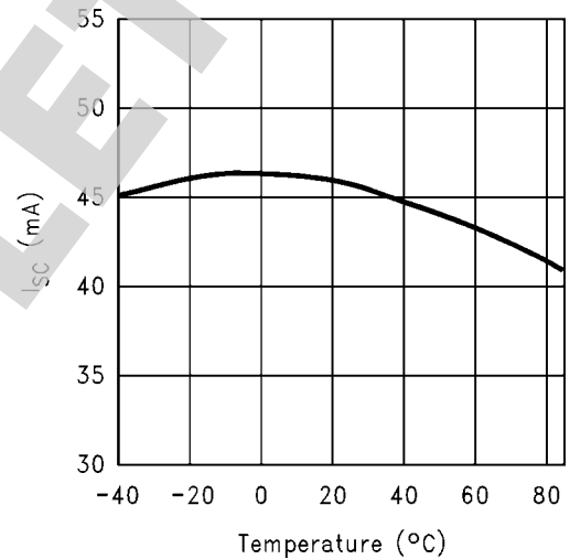
Short Circuit Current vs Temperature
