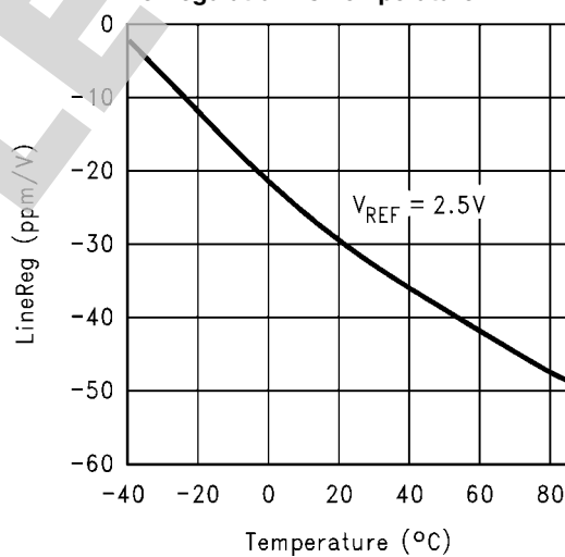
Line Regulation vs Temperature
