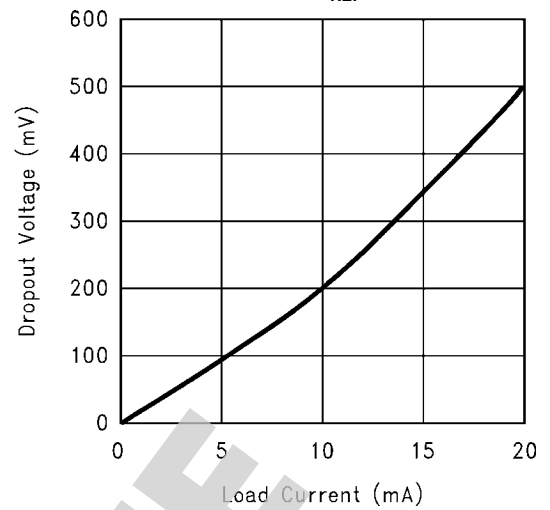
Dropout vs Load ( V_{REF} = 2.5 )
