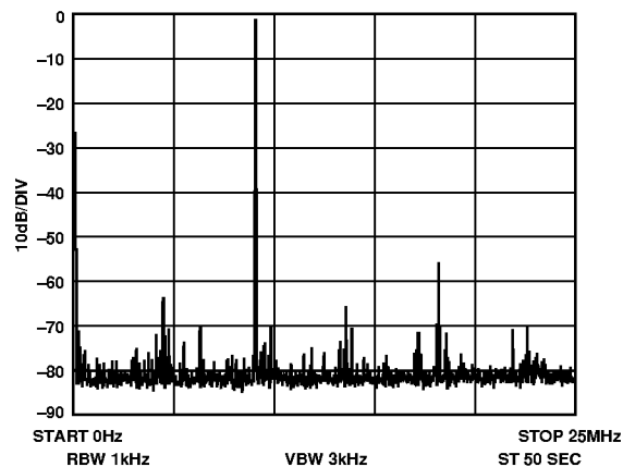
Figure 14. f_{MCLK} = 50 MHz, f_{OUT} = 9.1 MHz, Frequency Word = 2E978D50
