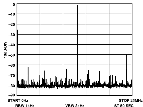
Figure 16. f_{MCLK} = 50 MHz, f_{OUT} = 13.1 MHz, Frequency Word = 43126E98
