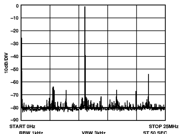
Figure 15. f_{MCLK} = 50 MHz, f_{OUT} = 11.1 MHz, Frequency Word = 38D4FDF4
