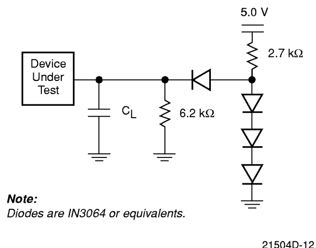
Figure 8. Test Setup
