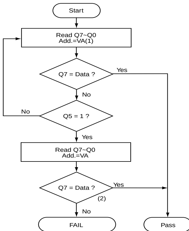
Figure 20. DATA# POLLING ALGORITHM
