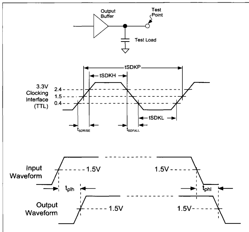
Figure 1. Clock Waveforms
