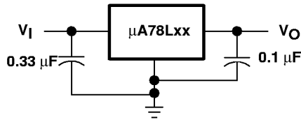
Figure 1. Fixed-Output Regulator
