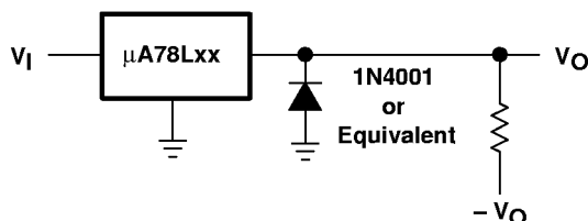
Figure 6. Output Polarity-Reversal Protection Circuit
