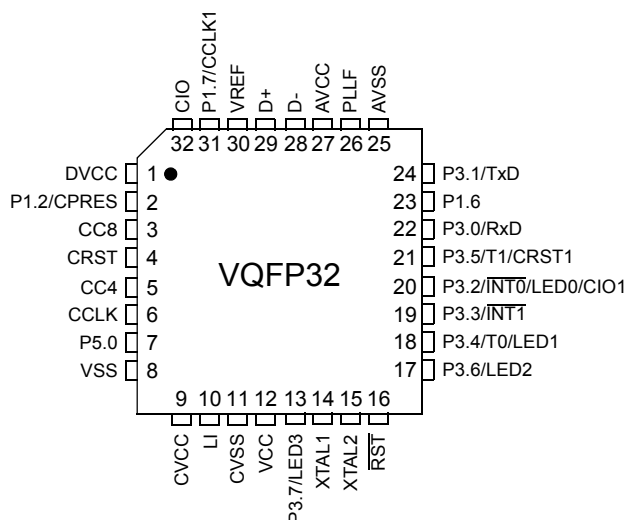
Figure 1. VQFP32 Package Pinout
