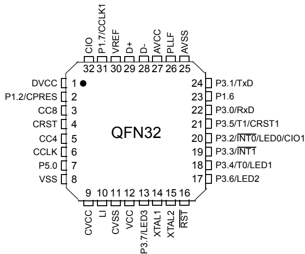
Figure 2. QFN32 Package Pinout
