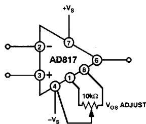
Figure 32. Offset Null Configuration
