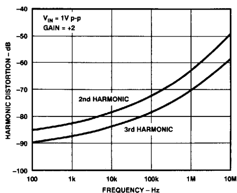
Figure 16. Harmonic Distortion vs. Frequency
