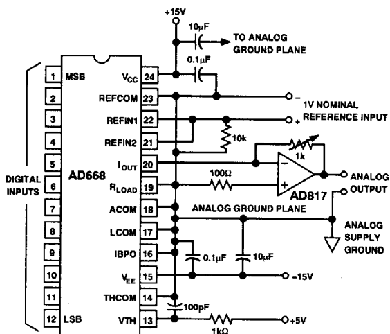
Figure 38. High Speed DAC Buffer
