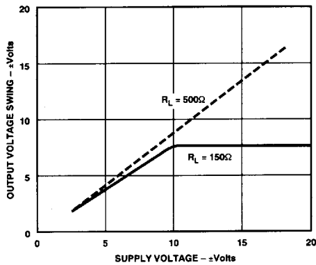
Figure 2. Output Voltage Swing vs. Supply
