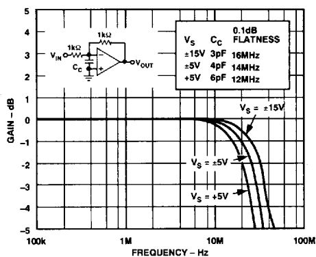
Figure 20. Closed-Loop Gain vs. Frequency, Gain = -1
