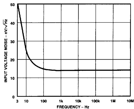
Figure 17. Input Voltage Noise Spectral Density
