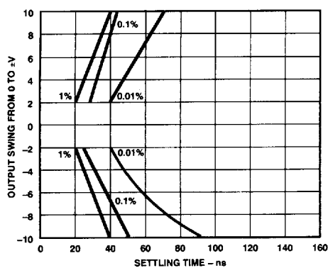
Figure 15. Output Swing and Error vs. Settling Time
