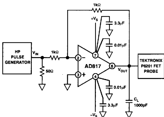
AD817 Driving a Large Capacitive Load
