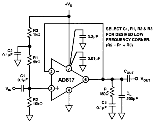
Figure 37. Single Supply Amplifier Configuration
