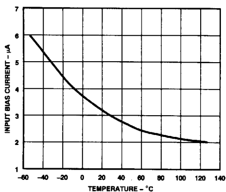
Figure 7. Input Bias Current vs. Temperature
