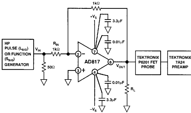
Figure 27. Inverting Amplifier Connection
