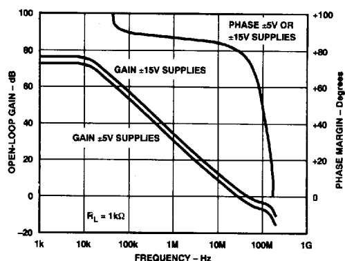
Figure 10. Open-Loop Gain and Phase Margin vs. Frequency
