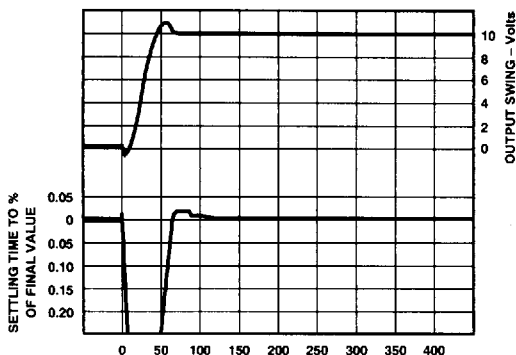
Figure 33. Settling Time in ns 0 V to +10 V
