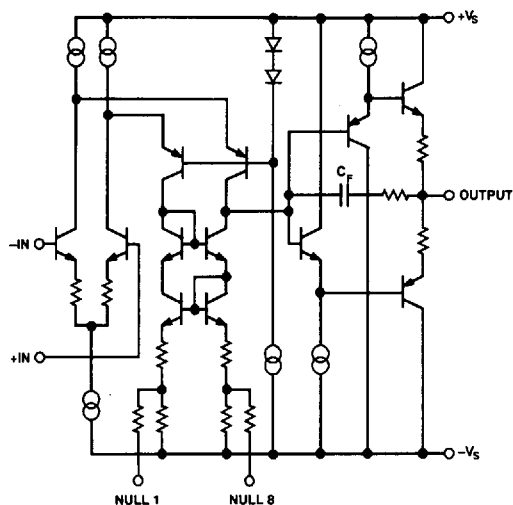
Figure 31. Simplified Schematic
