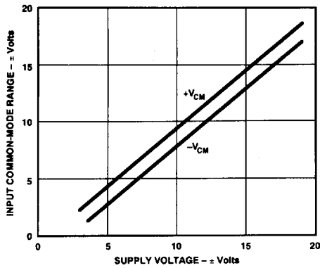
Figure 1. Common-Mode Voltage Range vs. Supply
