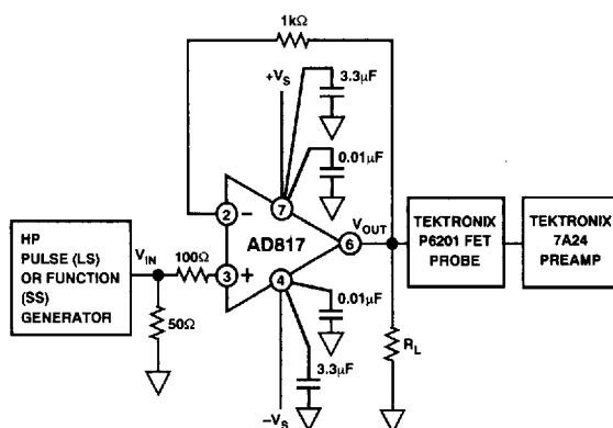
Figure 22. Noninverting Amplifier Connection
