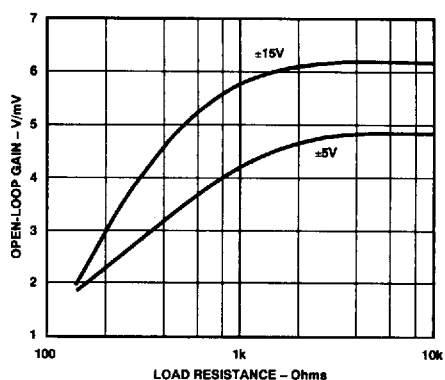
Figure 11. Open Loop Gain vs. Load Resistance
