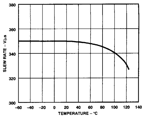
Figure 18. Slew Rate vs. Temperature
