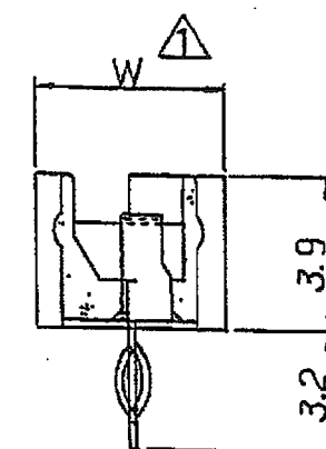
SECT. 断面 B'-B' (8P~12P)
