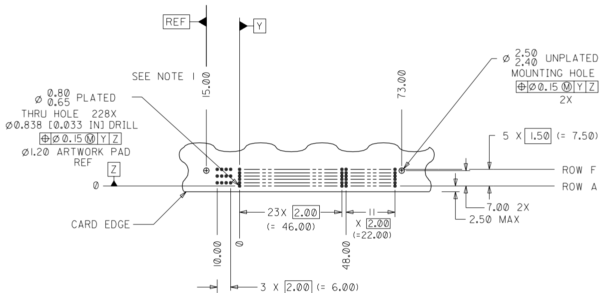
DAUGHTERCARD HOLE PATTERN AS VIEWED FROM CONNECTOR SIDE (NOTE THAT HOLE PATTERN HAS ITS OWN DATUM, SEPARATE FROM 3 VIEWS ON SHEET 1.)
