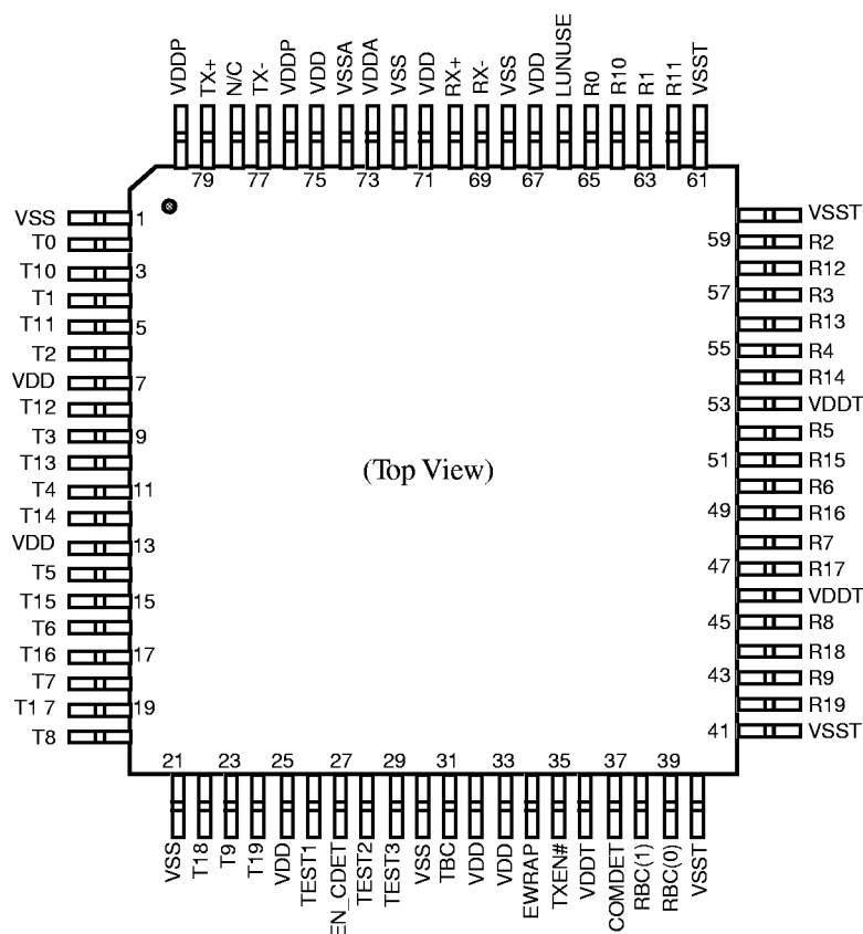
Figure 10: Pin Diagram
