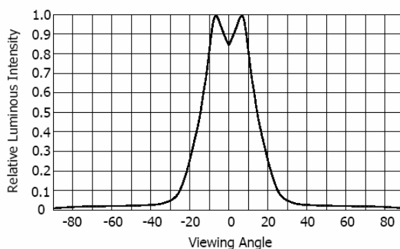
Fig.5a LTL914SxKS Relative Luminous Intensity vs. Viewing Angle
