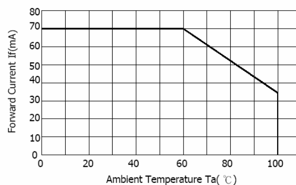
Fig.4 Forward Current vs. Ambient Temperature ( R_{\theta j-a}=300\text{ }^{\circ}\text{C/W} )
