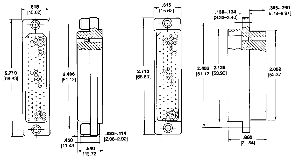
Receptacle Part Number 204027-2
