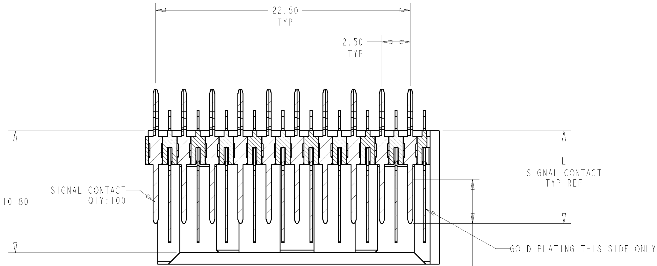
SECTION B-B
